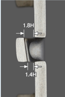
■ Cross Section (enlarged)
